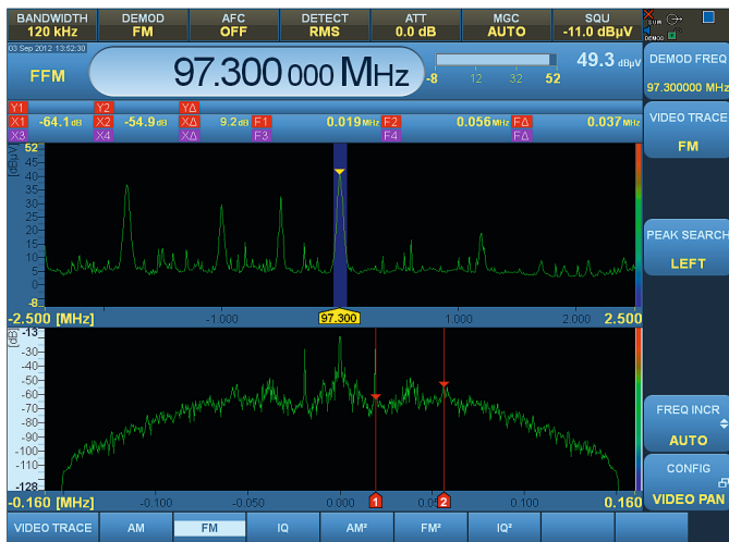
Display of the subcarriers of an FM radio signal using an FM-demodulated video spectrum (pilot tone: 19 kHz; RDS signal: 56 kHz from center frequency).
