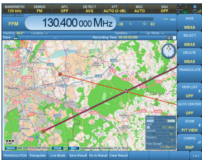
The positions recorded during a drive test (including the bearing, if applicable) are shown on a map.
